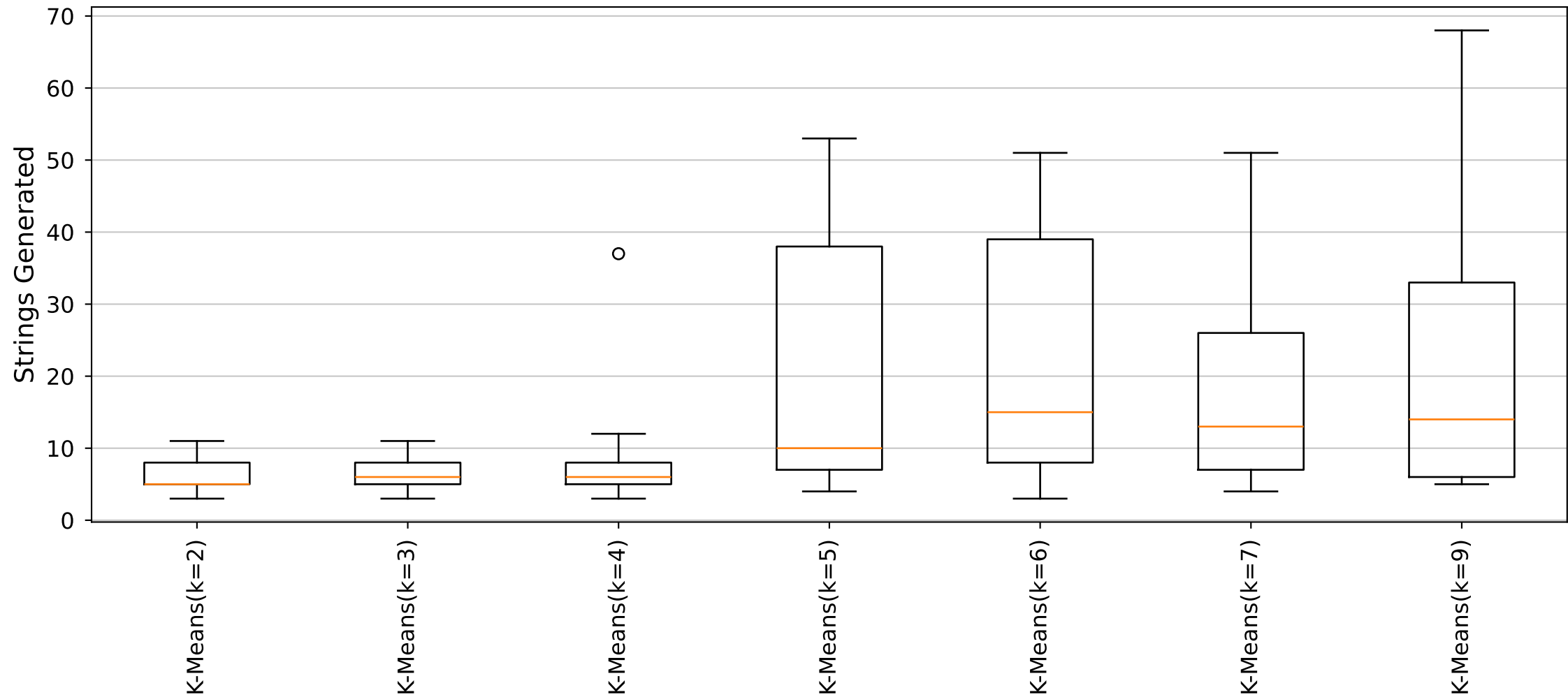
YARA Rules Strings Generated Distribution (Cluster11_Size9 dataset)
